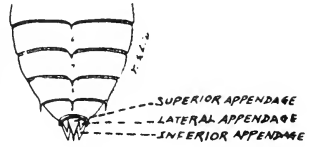
Fig. 144. Dorsal aspect of abdominal segments of a dragonfly naiad.
